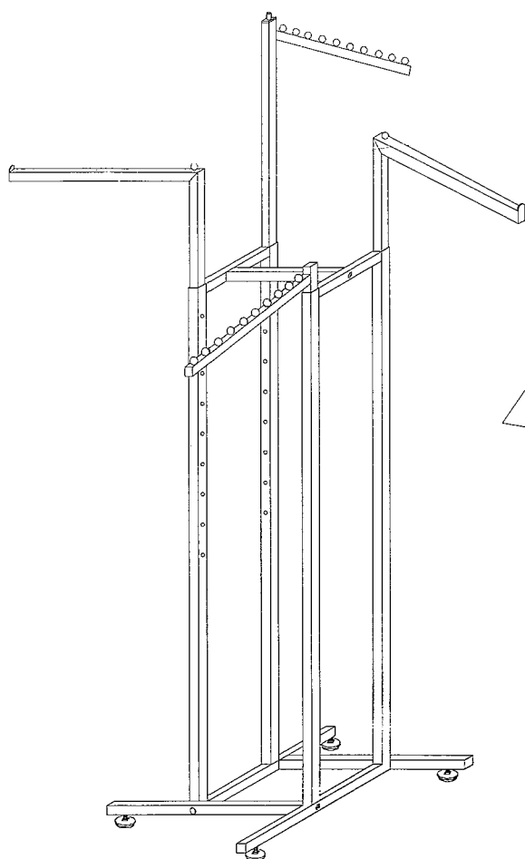
ASSEMBLY DRAWING
